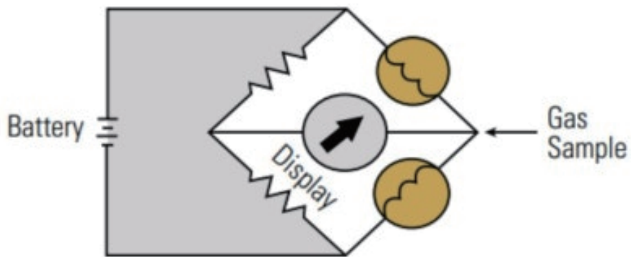
Wheatstone Bridge Circuit
