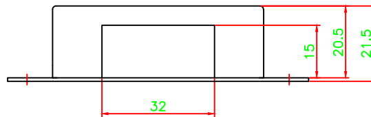
BOTTOM SIDE VIEW
